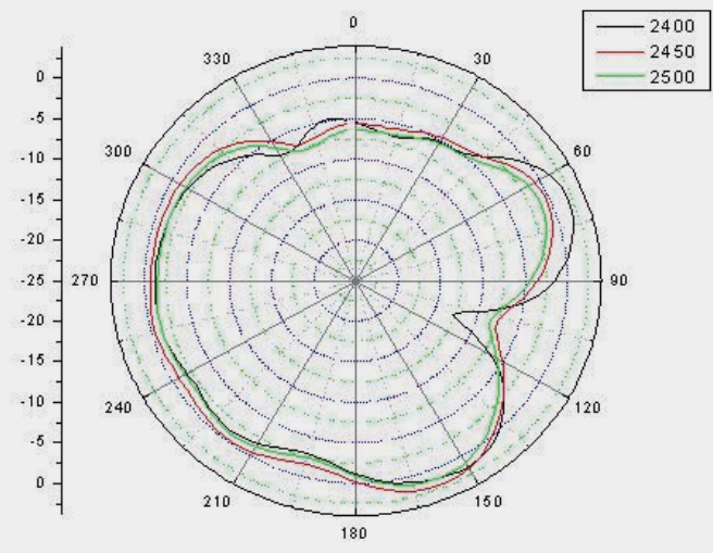
2.4G (PHI=90)
